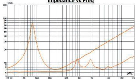
Impedance vs Freq
